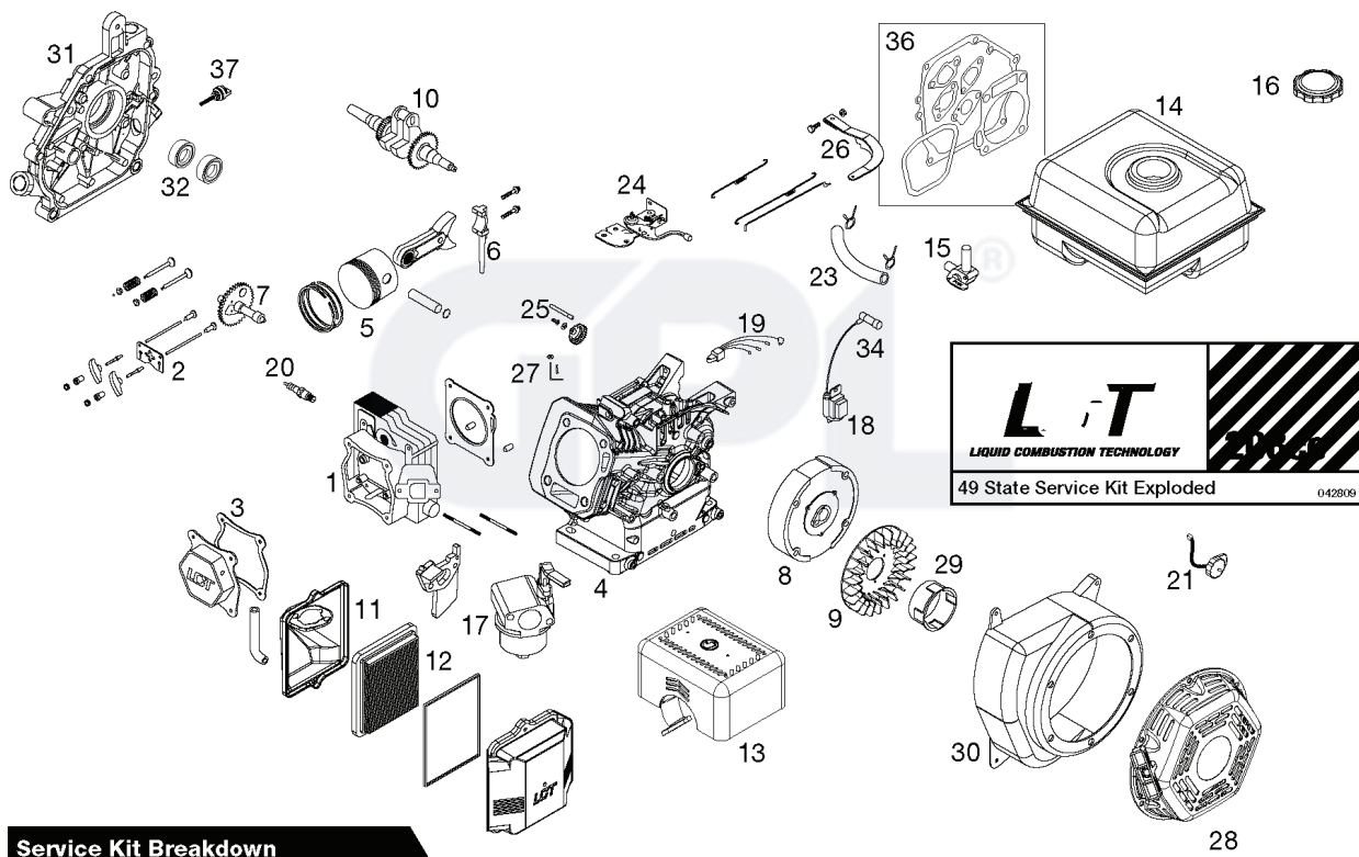
Service Kit Breakdown
