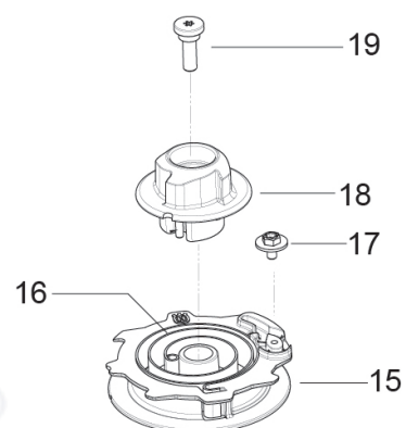
EPS (SLOW PULL) STARTER ASSEMBLY DETAIL
