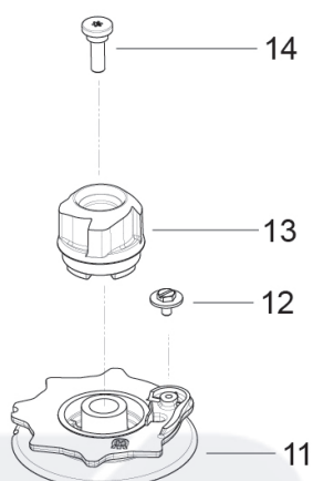
TWO PIECE STANDARD STARTER ASSEMBLY DETAIL
