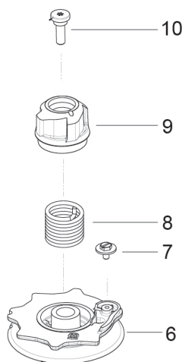
SPRING ASSIST STARTER ASSEMBLY DETAIL
