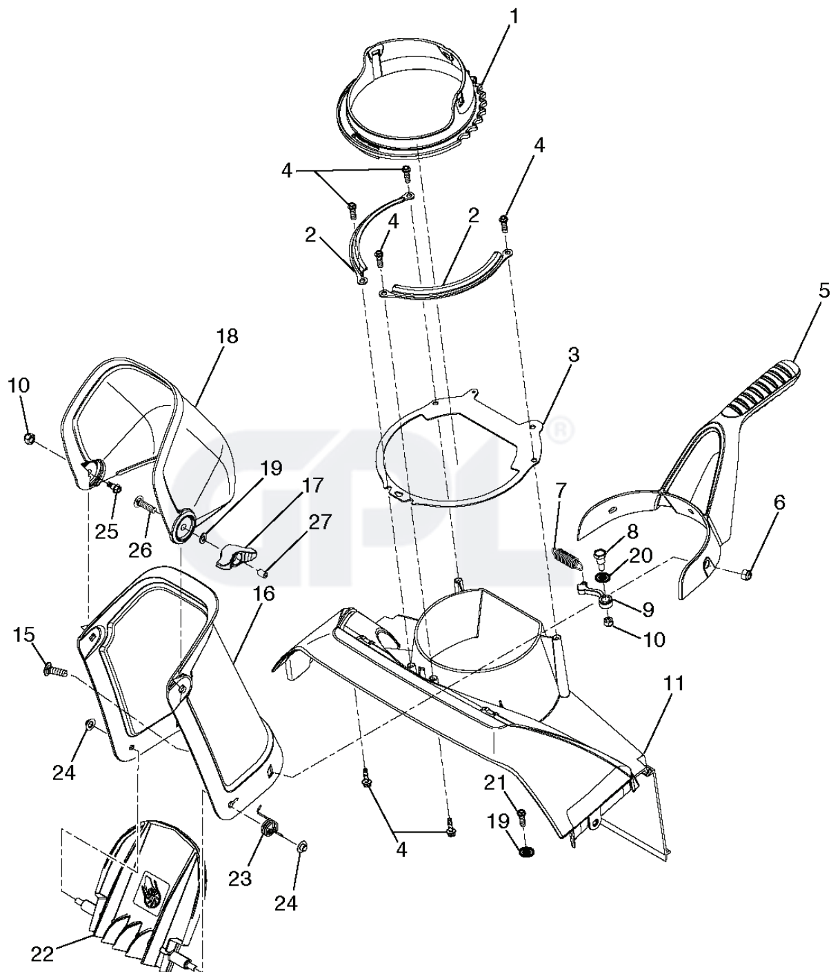
SSST-Chute asm_12
