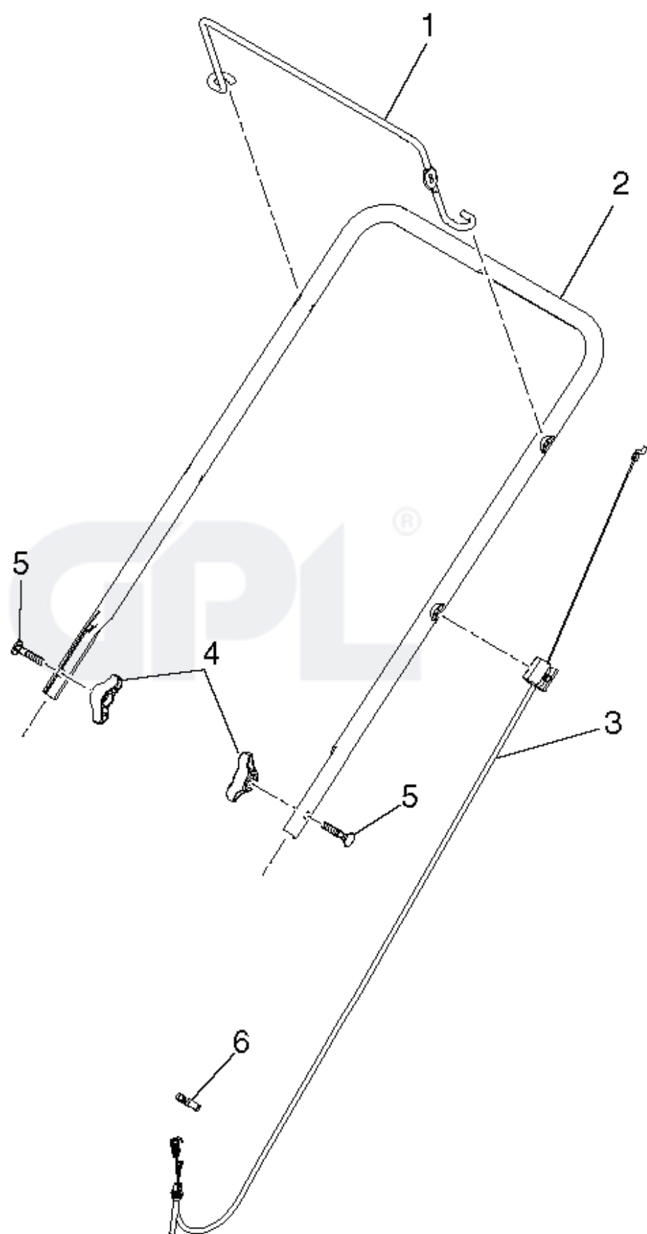
SSST-Handle asm_1
